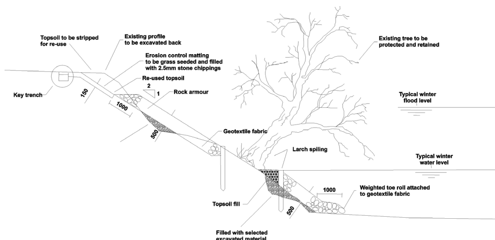
Figure 8.48 Revetment incorporating mature tree (courtesy Mott MacDonald)
