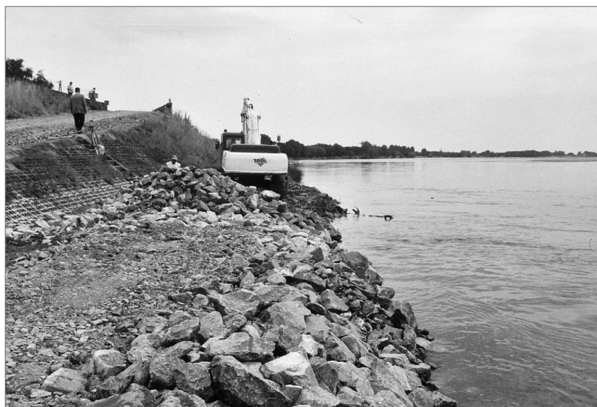
Figure 8.14 Flood protection dike along the Loire river under rehabilitation, notably the scour protection (courtesy TPPL France)
