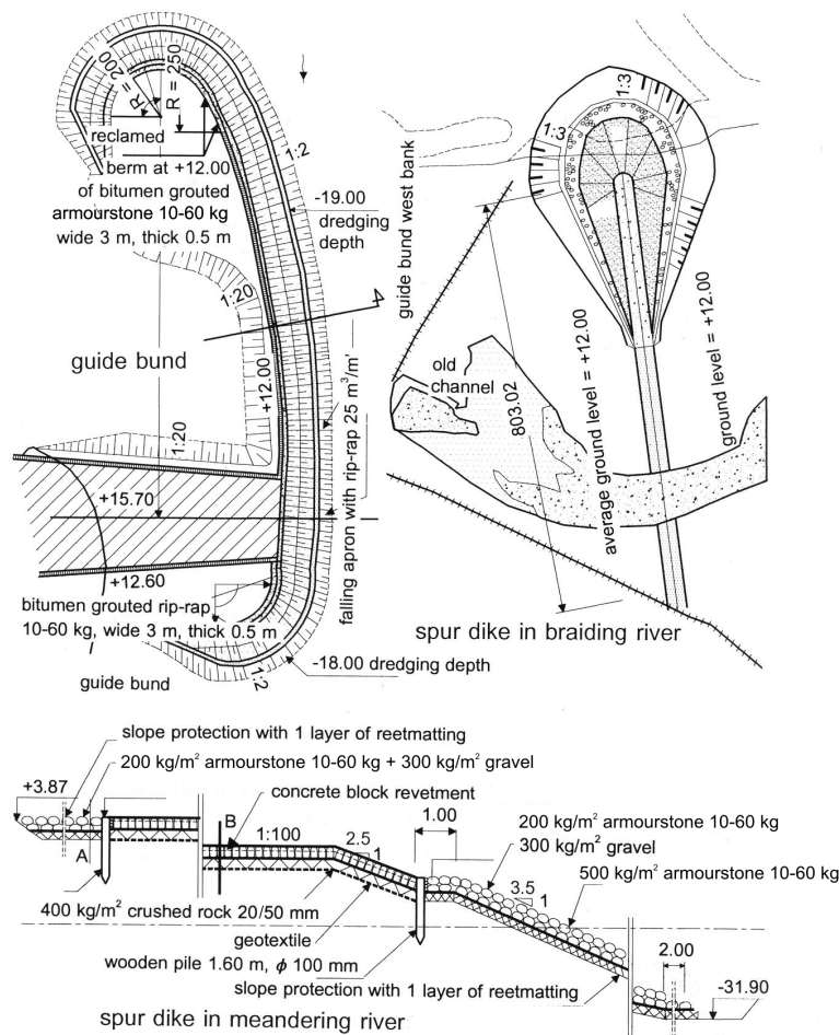
Figure 8.25 Examples of heads of spur-dikes and end of guide bunds
