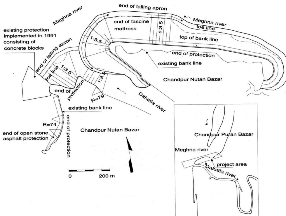
Figure 8.15 Example of a suite of structures in a braided river (courtesy Royal Haskoning)
