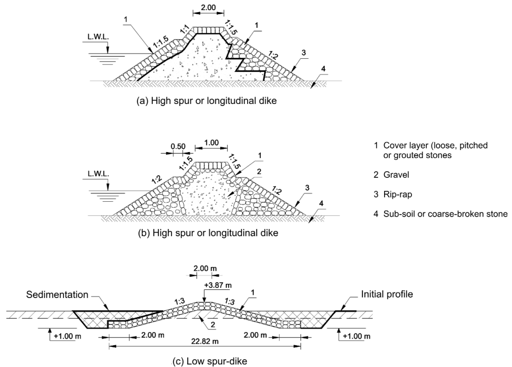
Figure 8.23 Typical cross-sections of dikes
