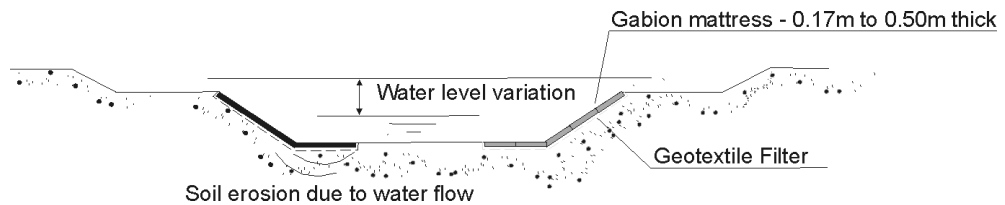
Figure 8.53 Partial or total lining of the section (courtesy Maccaferri, France)
