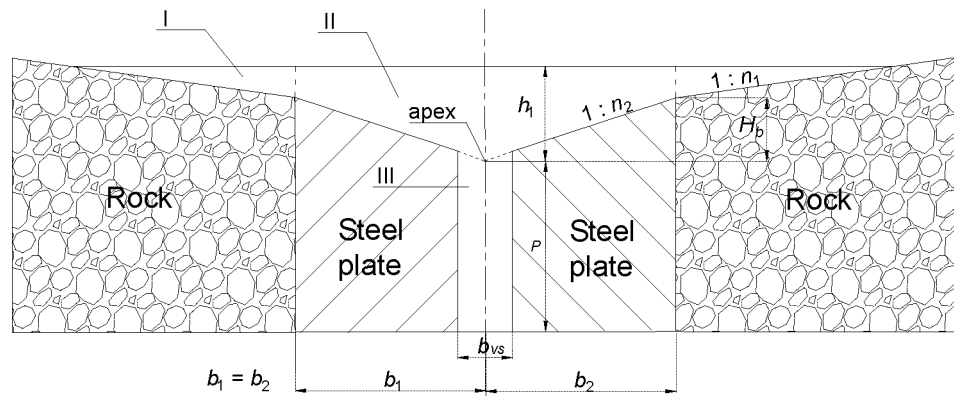
Figure 8.50 Cross section of the V-shaped weir with vertical slot (courtesy Rijkswaterstaat)
