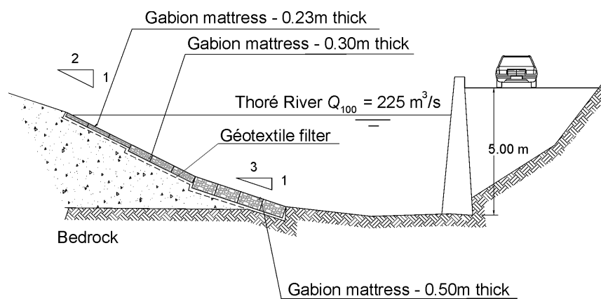
Figure 8.54 Thickening of revetment to provide adequate toe protection (River Thoré, France) (courtesy Maccaferri, France)
