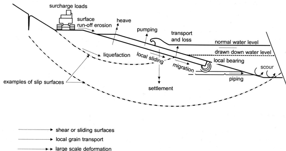
Figure 8.22 Riverbank subsoil failure mechanisms
