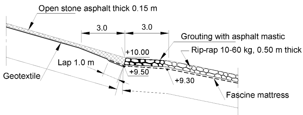
Figure 8.32 Transition from penetrated or grouted stone to rip-rap. Asphalt grouting is preferably done above the water level (dimensions in m)
