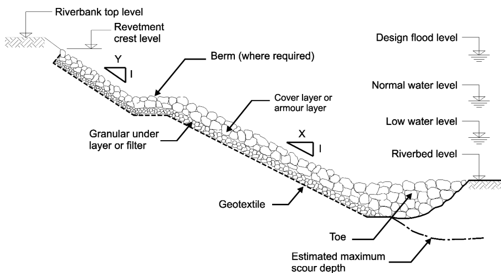
Figure 8.10 Components of a typical armourstone revetment
