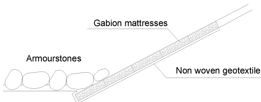
Figure 8.57 Transition between gabion revetment and armourstone (courtesy Maccaferri, France)
