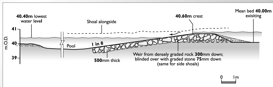
Figure 8.47 Cross-section through the weir
