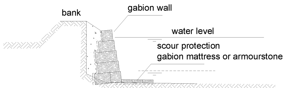
Figure 8.55 Typical cross-section for gabion wall bank protection (courtesy Maccaferri, France)
