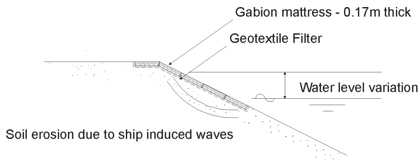
Figure 8.52 Use of gabion mattresses for protection against waves of the upper part of the bank (courtesy Maccaferri, France)
